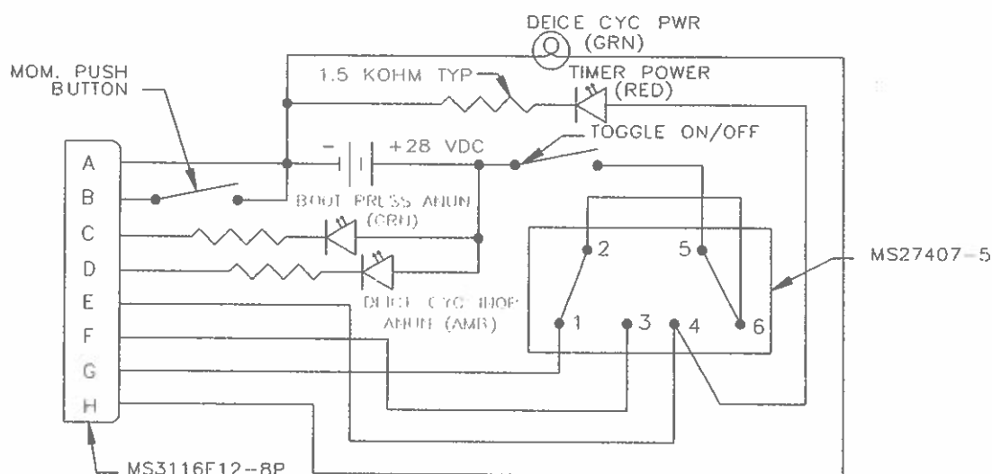
Deice Cycler Test Box Wiring Diagram
