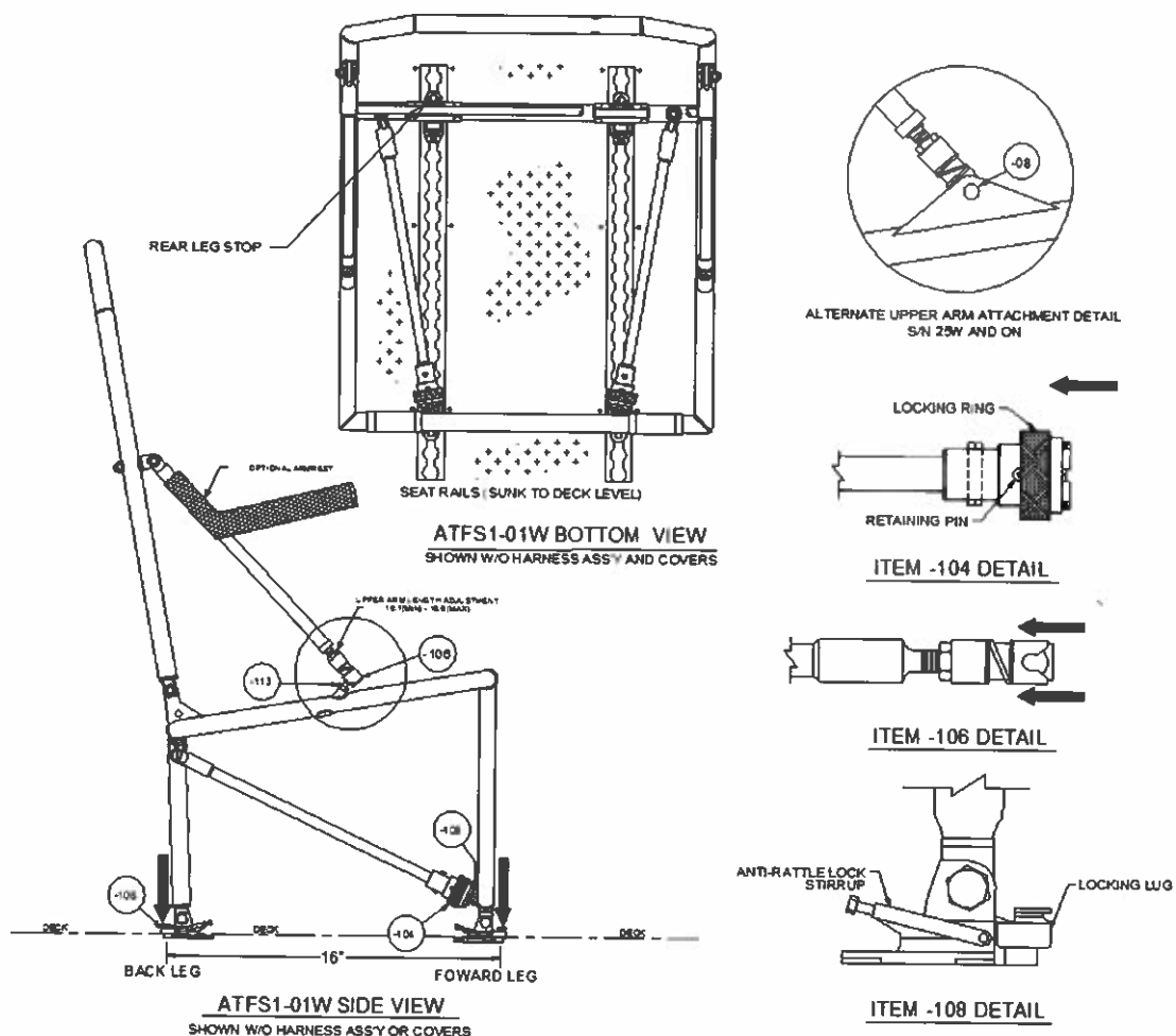
Figure 1.2.1 Seat Installation
