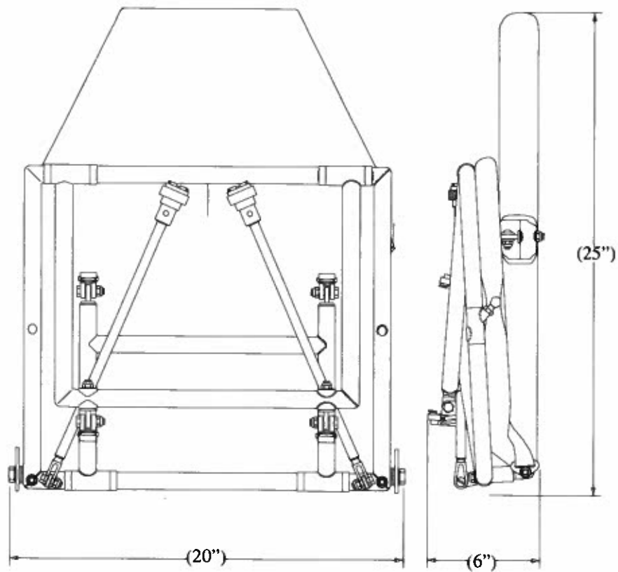
Figure 1.1.2 Folded Seat Dimensions
