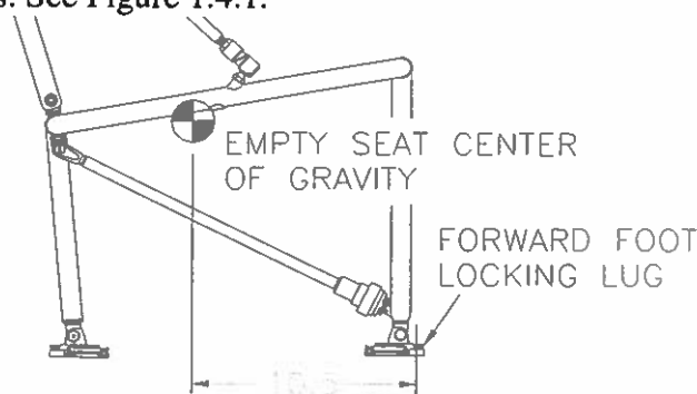
Figure 1.4.1: Empty Seat Center of Gravity Location
