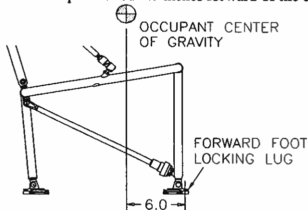
Figure 1.4.2: Occupant C.G. Position
