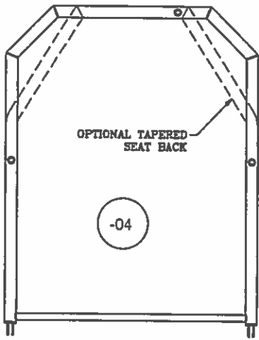
PN ATFS1-04, SEAT BACK ASS'Y WELDMENT
