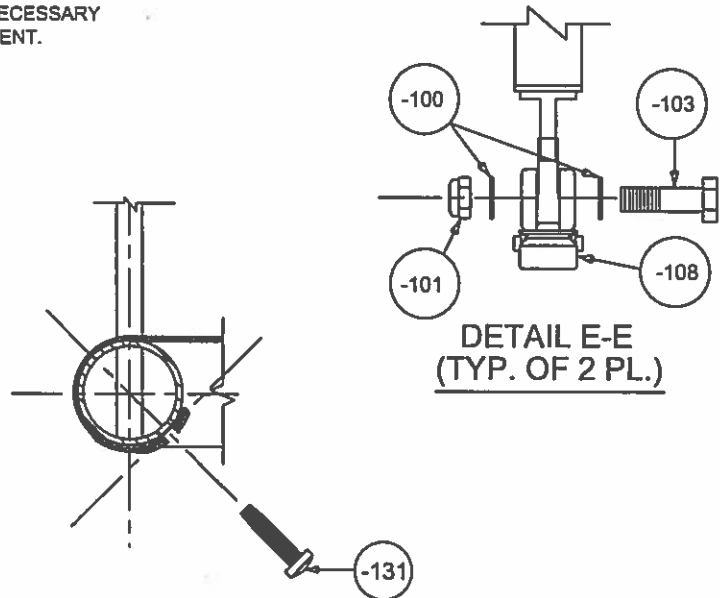
DETAIL F-F (TYP. OF 20 PL. THRU S/N 1599) (TYP. OF 18 PL. S/N 1600 AND ON)
