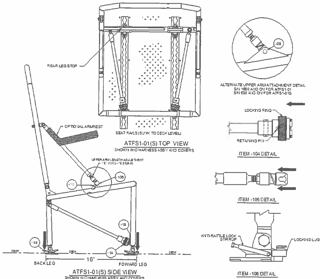
Figure 1.2.1 Seat Installation
