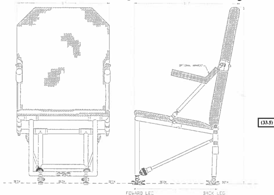
Figure 1.1.1 Basic Seat Dimensions
