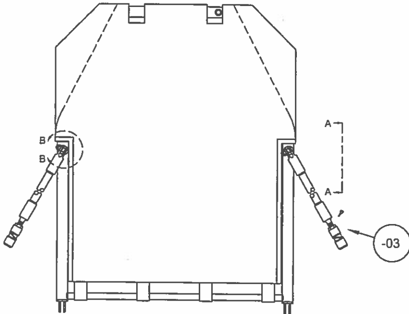
PN ATFS1-04, SEAT BACK ASS'Y WELDMENT
